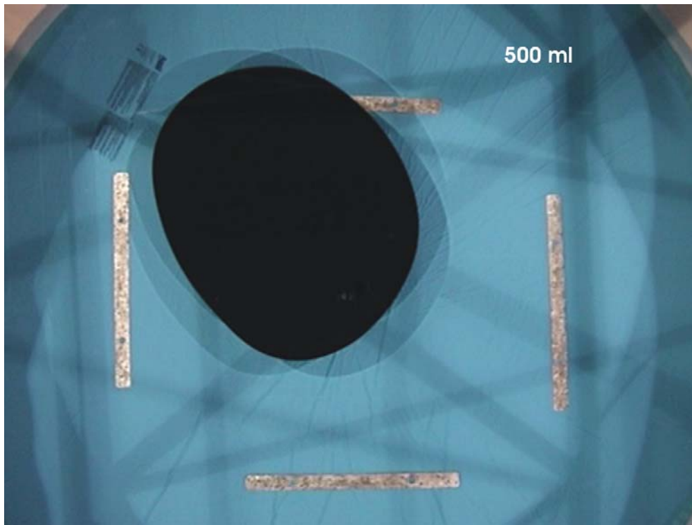
Figure 2. Initial spreading of oil on water API 25
